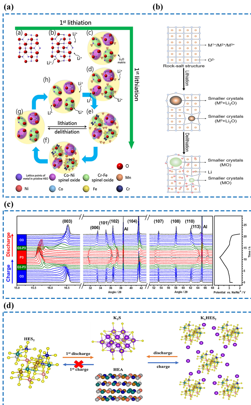
Fig. 5 a Schematic illustration of atomic-scale microstructure evolution of (\text{CrMnFeCoNi})_3\text{O}_4 HEO during lithiation/delithiation cycling [159], Copyright 2021, Elsevier. b Schematic diagram of the structural transition of the lithiation/de-lithiation of (\text{MgCoNiCuZn})\text{O} HEO anodes for LIBs [247], Copyright 2023, Elsevier. c Operando XRD patterns and the corresponding voltage curve of the \text{NaCu}_{0.1}\text{Ni}_{0.3}\text{Fe}_{0.2}\text{Mn}_{0.2}\text{Ti}_{0.2}\text{O}_2 (NCNFMT) electrode during the first cycle at 0.1C, in the voltage range of 2.0–3.9 V vs. \text{Na}/\text{Na}^+ [201], Copyright 2022, Elsevier. d Schematic illustration of the reaction mechanism of \text{HES}_2 [248], Copyright 2023, Elsevier
