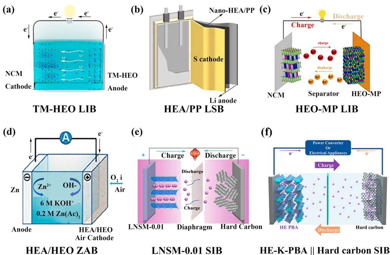
Fig. 4 Schematic figure of a full-cell using NCM111 cathode and TM-HEO anode for LIB [187], Copyright 2019, Elsevier; b pouch cell of LSB [137], Copyright 2021, Elsevier; c full-cell of HEO-MP LIB [204], Copyright 2022, Elsevier; d HEA/HEO ZAB [240], Copyright 2020, American Chemical Society; e LNSM-0.01 SIB [241], Copyright 2023, Elsevier; f HE-K-PBA||Hard carbon SIB [202], Copyright 2023, American Chemical Society
