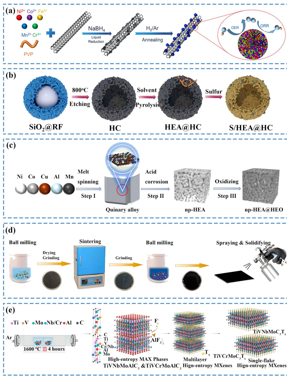
Fig. 3 Schematic diagram of preparation process of a \text{Fe}_{12}\text{Ni}_{23}\text{Cr}_{10}\text{Co}_{55-x}\text{Mn}_x/\text{CNT} and principle of bifunctional ORR/OER [93], Copyright 2023, American Chemical Society. b \text{S/HEA@HC} [117], Copyright 2024, American Chemical Society. c \text{np-HEA@HEO} [119], Copyright 2023, Elsevier. d Ball milling process of (\text{Cu}, \text{Mn}, \text{Fe}, \text{Cr})_3\text{O}_4 [121], Copyright 2022, American Chemical Society. e HE MAX and MXenes [33], Copyright 2021, American Chemical Society
