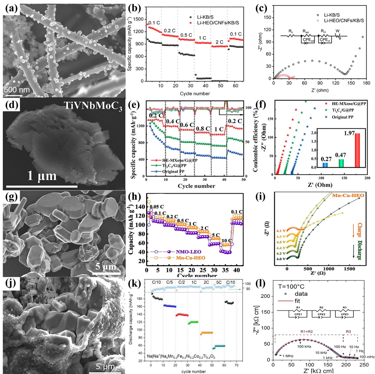
Fig. 6 a SEM images of grapevine-like HEO composite, b Li-KB/S, and Li-HEO/CNFs/KB/S for LSBs, and c EIS plots with and without HEO/CNFs interlayers [276], Copyright 2024, Elsevier. d SEM images of \text{TiVNbMoC}_3 , e HE MXene/G@PP, \text{Ti}_3\text{C}_2/\text{G@PP} , and original PP for LSBs, and f EIS and inset illustrate the lithium-ion conductivity of the cells with pristine PP, \text{Ti}_3\text{C}_2/\text{G@PP} , and HE MXene/G@PP [277], Copyright 2024, American Chemical Society. g SEM images of high-entropy Mn-Cu-HEO, h Mn-Cu-HEO, and NMO-LEO for SIBs, and i Nyquist plots of Mn-Cu-HEO cathode [279], Copyright 2023, Elsevier. j SEM images of \text{NaMn}_{0.2}\text{Fe}_{0.2}\text{Co}_{0.2}\text{Ni}_{0.2}\text{Ti}_{0.2}\text{O}_2 , k the first cycle of charging/discharging of \text{NaMn}_{0.2}\text{Fe}_{0.2}\text{Co}_{0.2}\text{Ni}_{0.2}\text{Ti}_{0.2}\text{O}_2 , and l the frequency response of the sample measured at 100 °C presented as a Nyquist. Inset illustrates the equivalent circuit used for fitting the frequency response [280], Copyright 2022, Elsevier
